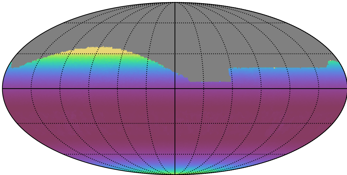
no_long_daily_v3.4_10yrs All sky r band: Min airmass
