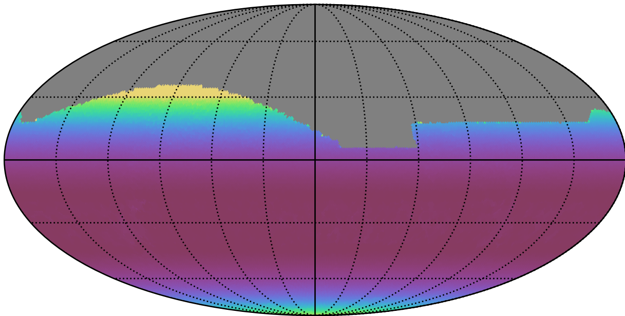
no_long_daily_v3.4_10yrs All sky i band: Min airmass
