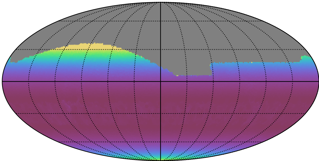
no_long_daily_v3.4_10yrs All sky g band: Min airmass
