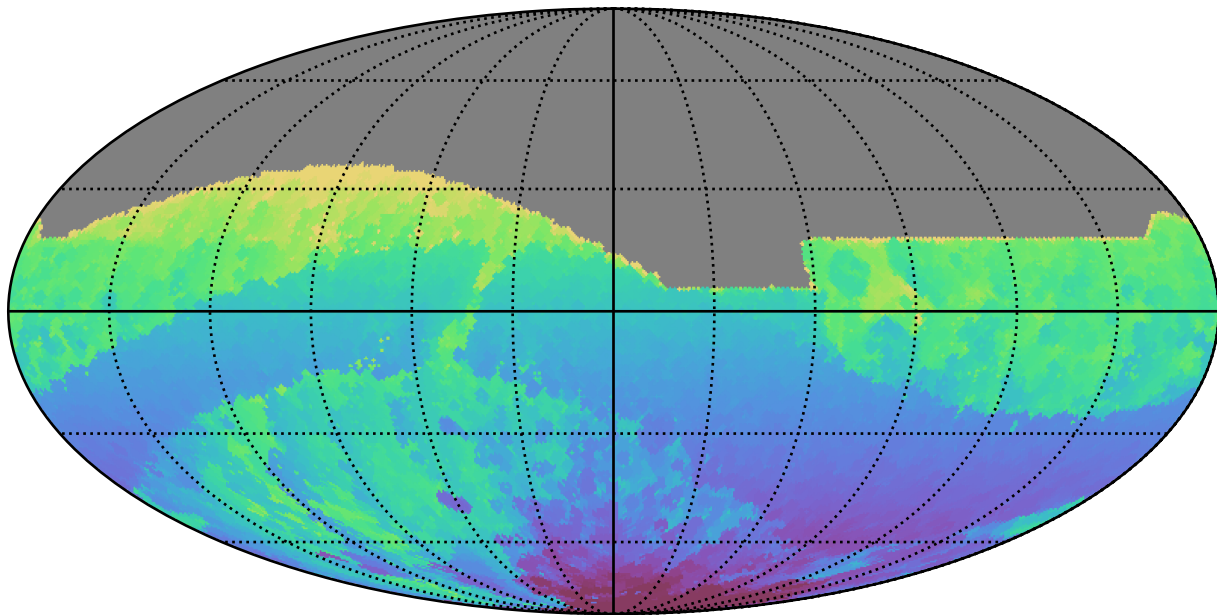
no_long_daily_v3.4_10yrs All sky all bands: Min HA
