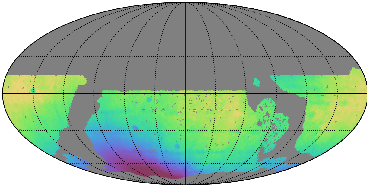
no_long_daily_v3.4_10yrs WFD all bands: Median solarElong
