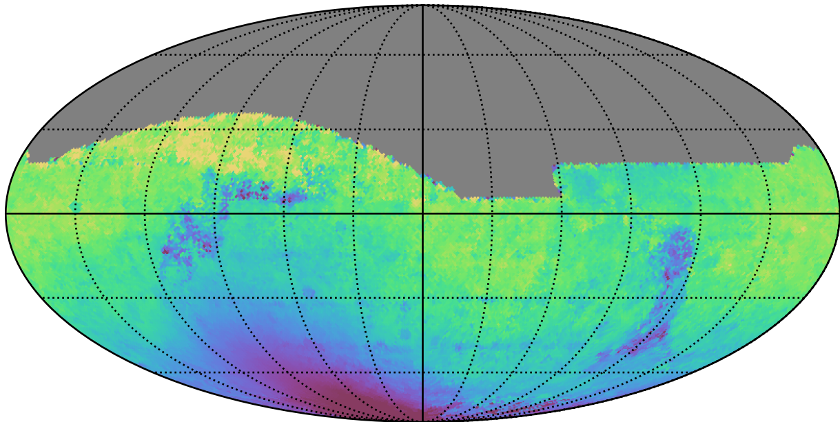
no_long_daily_v3.4_10yrs All sky z band: Median solarElong
