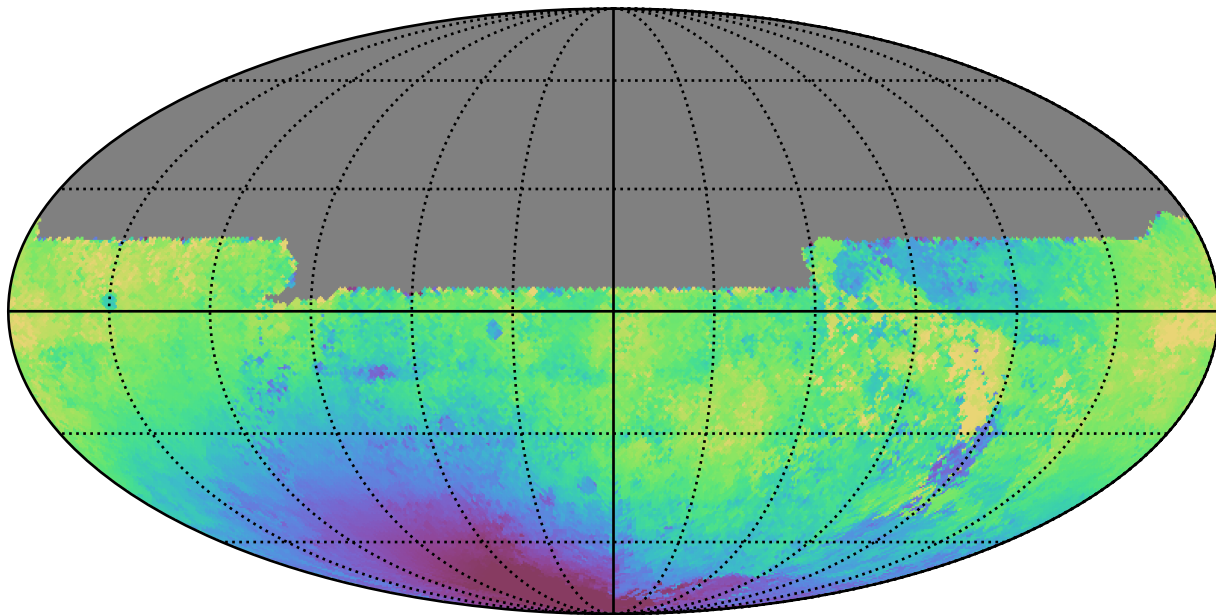
no_long_daily_v3.4_10yrs All sky u band: Median solarElong
