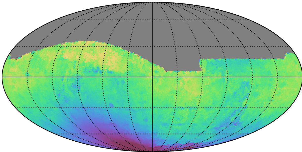
no_long_daily_v3.4_10yrs All sky i band: Median solarElong
