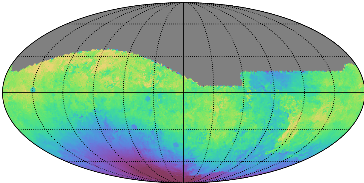
no_long_daily_v3.4_10yrs All sky g band: Median solarElong
