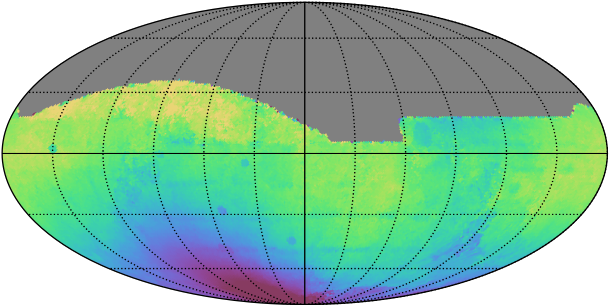
no_long_daily_v3.4_10yrs All sky all bands: Median solarElong
