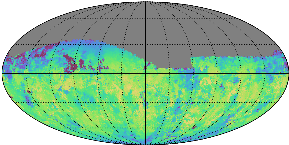
no_long_daily_v3.4_10yrs Yr 1 z band: Median skyBrightness
