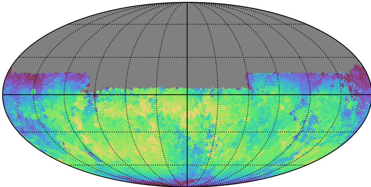
no_long_daily_v3.4_10yrs Yr 1 y band: Median skyBrightness
