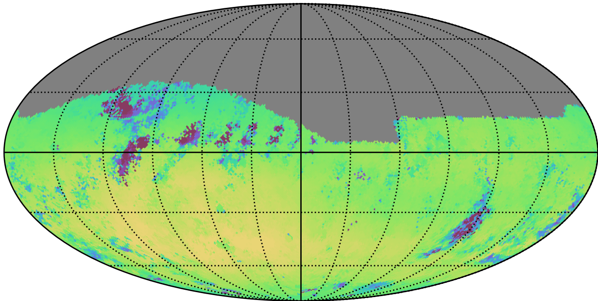
no_long_daily_v3.4_10yrs Yr 1 r band: Median skyBrightness
