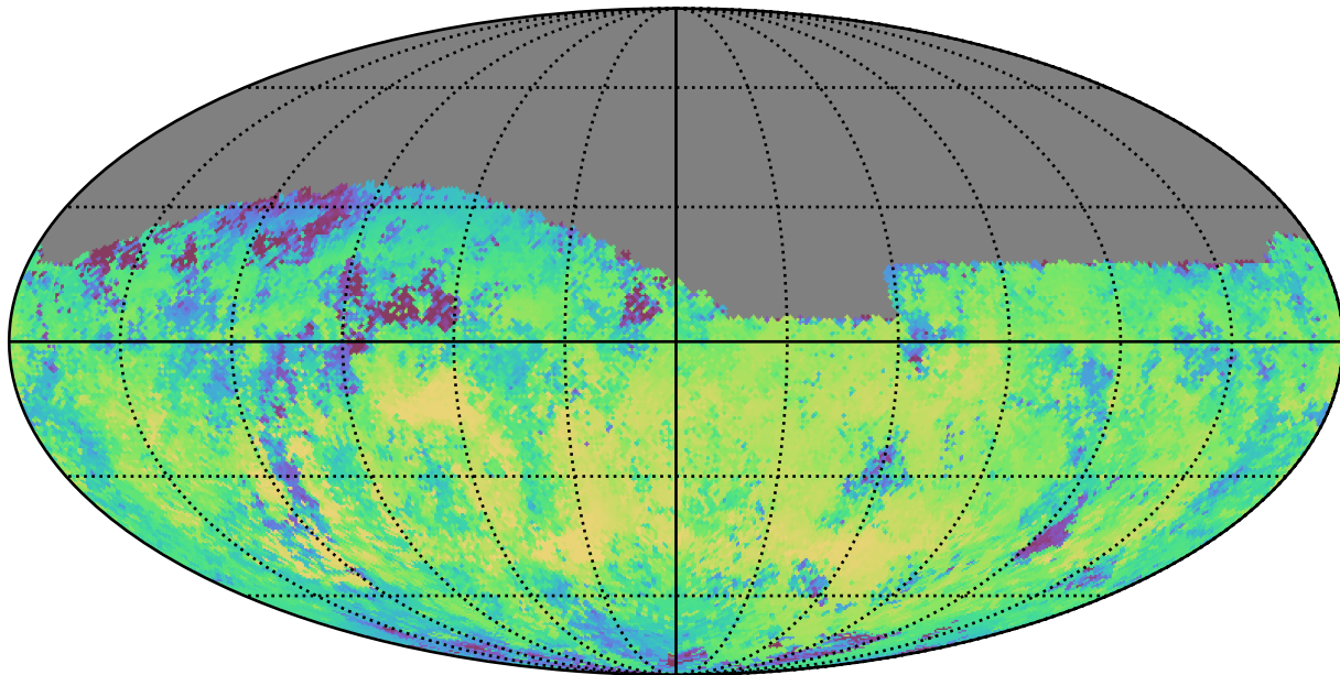
no_long_daily_v3.4_10yrs Yr 1 i band: Median skyBrightness
