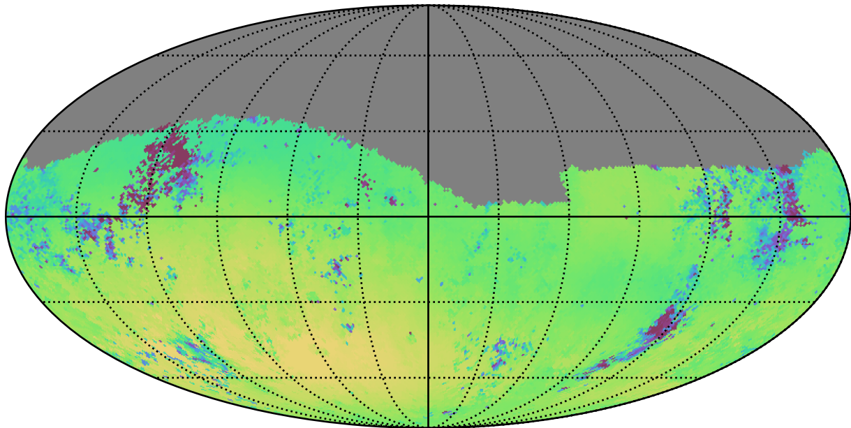
no_long_daily_v3.4_10yrs Yr 1 g band: Median skyBrightness
