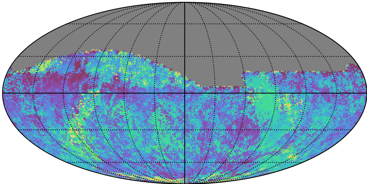
no_long_daily_v3.4_10yrs Yr 1 all bands: Median skyBrightness
