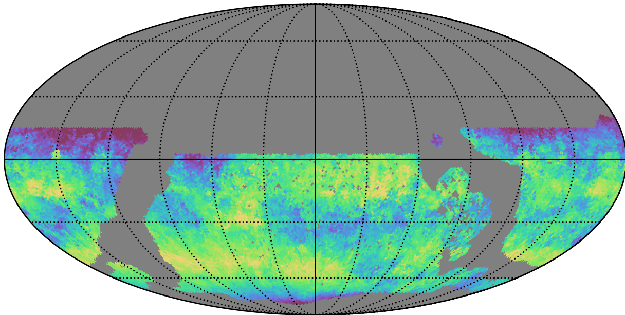
no_long_daily_v3.4_10yrs WFD z band: Median skyBrightness
