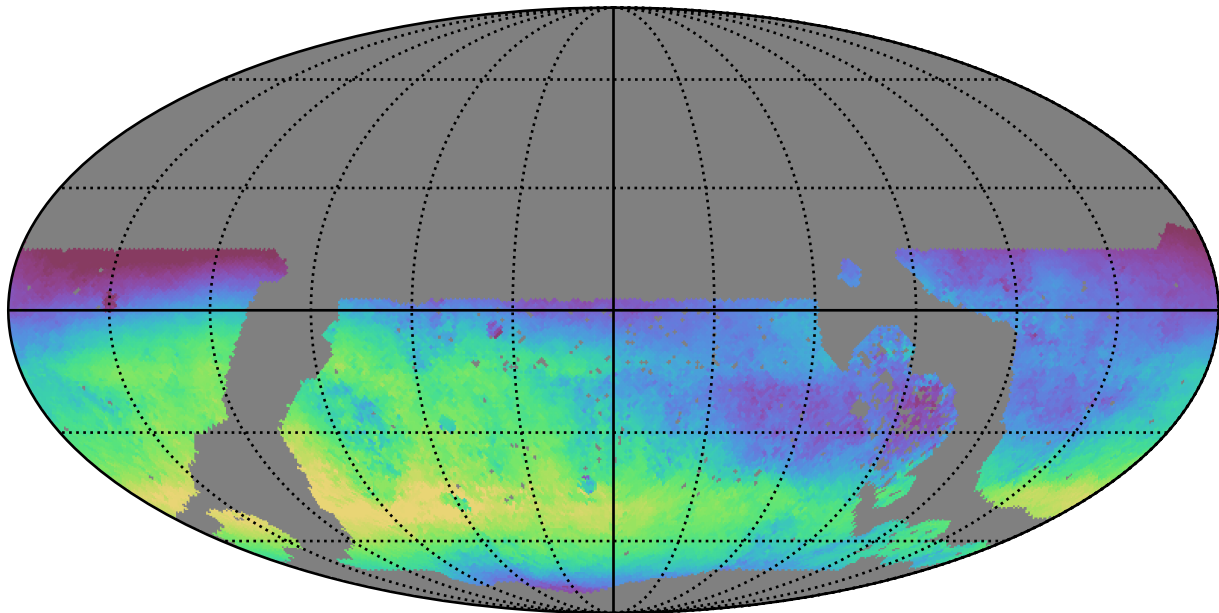
no_long_daily_v3.4_10yrs WFD u band: Median skyBrightness
