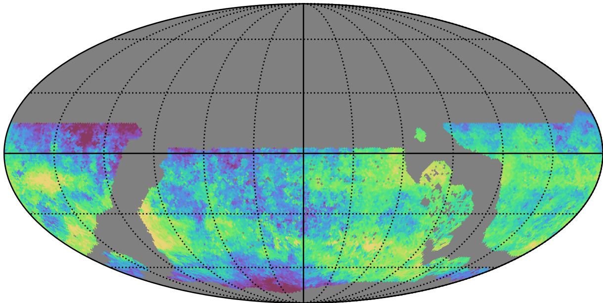
no_long_daily_v3.4_10yrs WFD i band: Median skyBrightness
