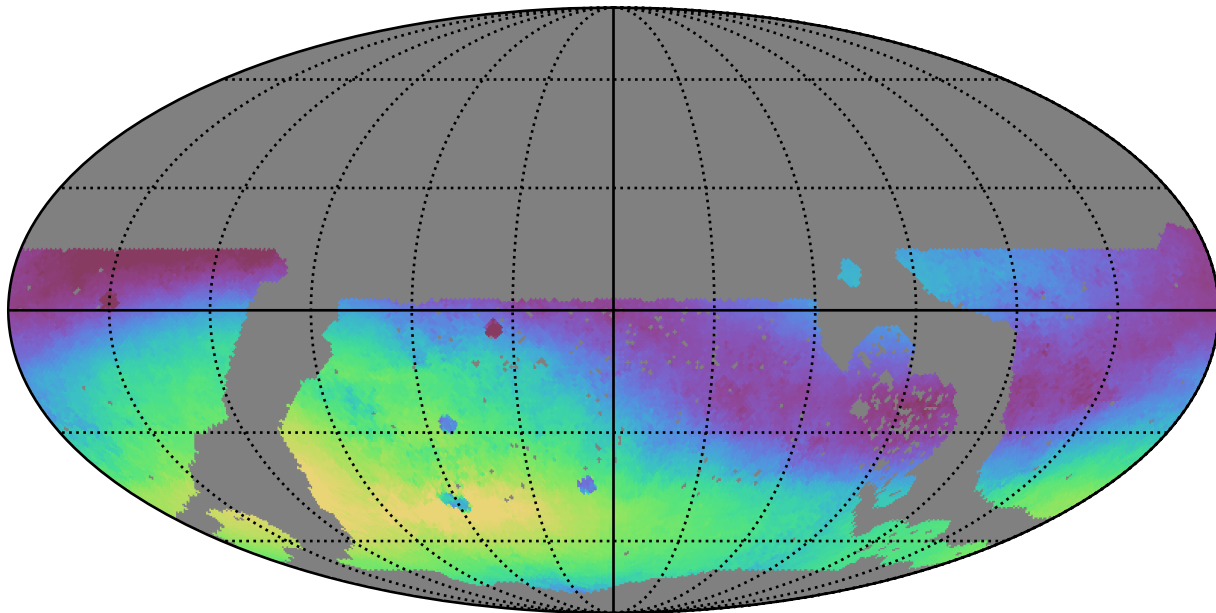
no_long_daily_v3.4_10yrs WFD g band: Median skyBrightness
