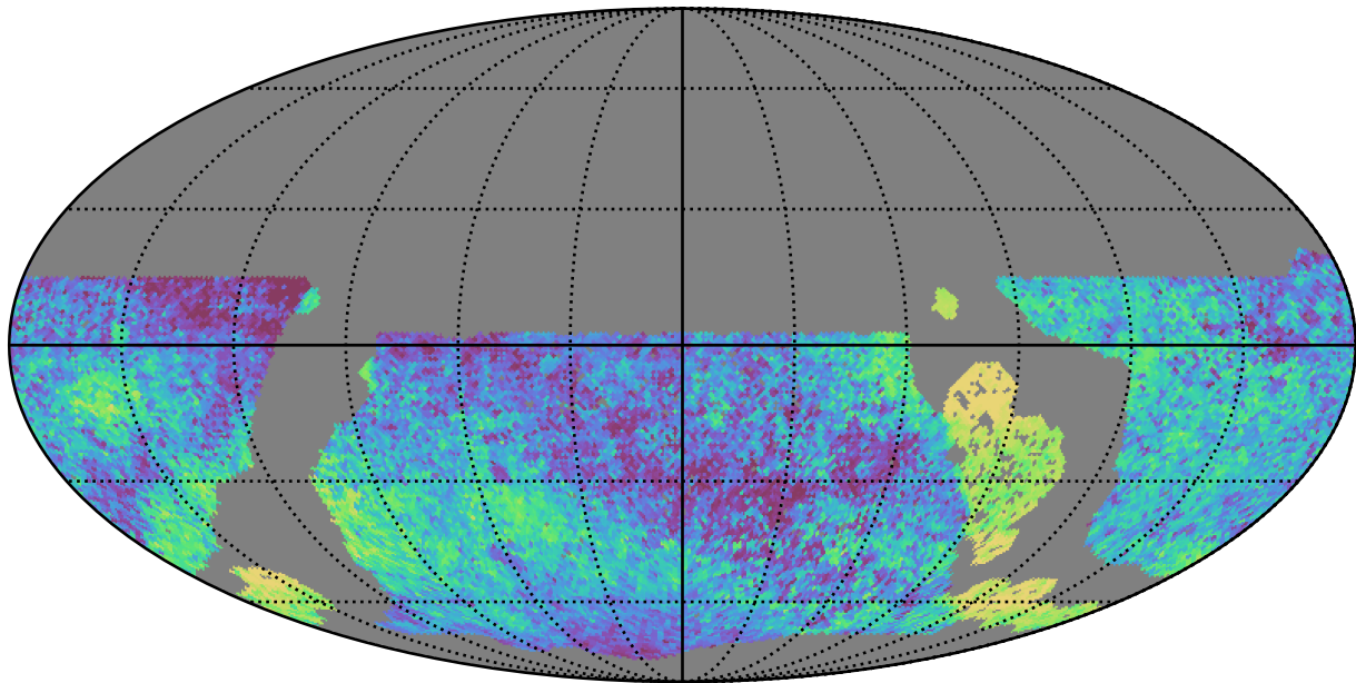
no_long_daily_v3.4_10yrs WFD all bands: Median skyBrightness
