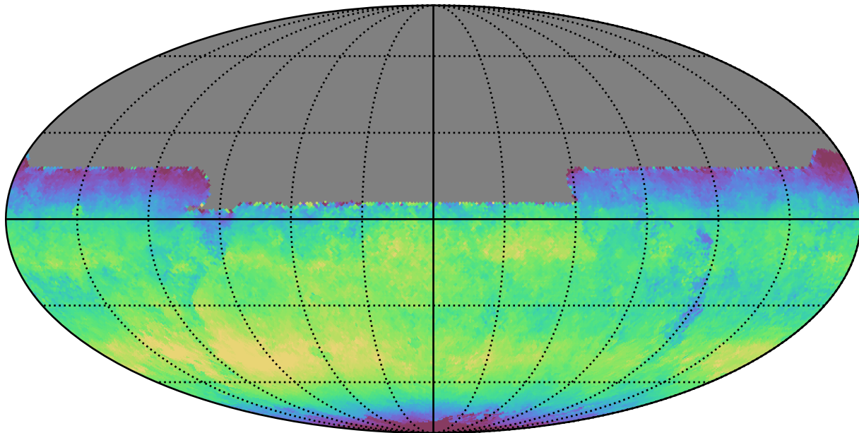
no_long_daily_v3.4_10yrs All sky y band: Median skyBrightness
