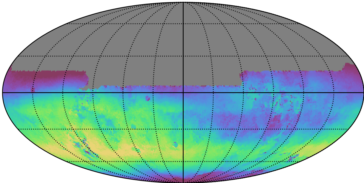
no_long_daily_v3.4_10yrs All sky u band: Median skyBrightness
