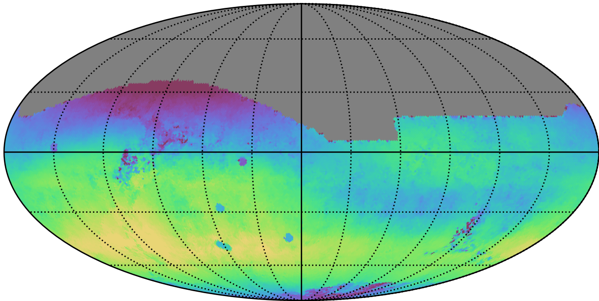
no_long_daily_v3.4_10yrs All sky r band: Median skyBrightness
