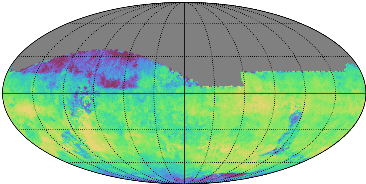
no_long_daily_v3.4_10yrs All sky i band: Median skyBrightness
