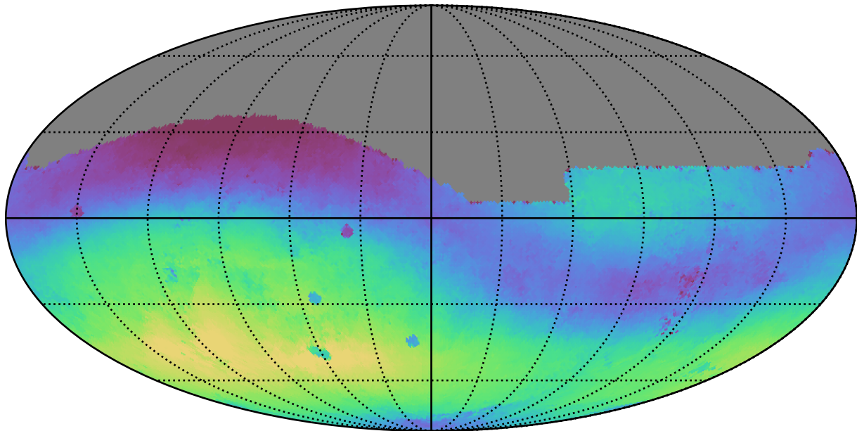
no_long_daily_v3.4_10yrs All sky g band: Median skyBrightness
