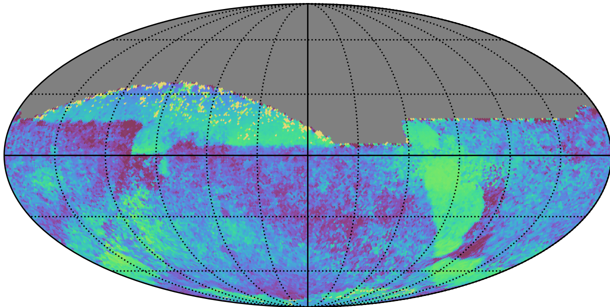
no_long_daily_v3.4_10yrs All sky all bands: Median skyBrightness
