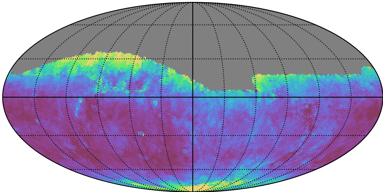
no_long_daily_v3.4_10yrs Yr 1 all bands: Median seeingGeom
