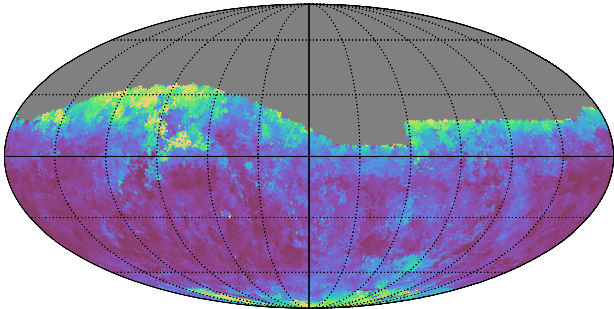
no_long_daily_v3.4_10yrs Yr 1 i band: Median seeingEff
