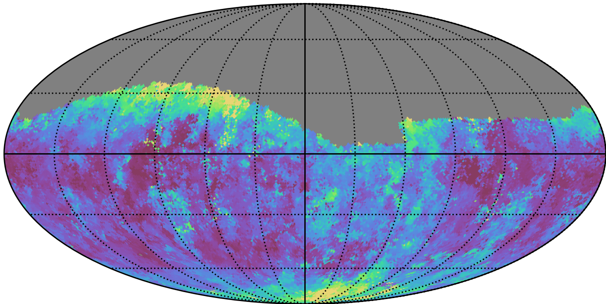
no_long_daily_v3.4_10yrs Yr 1 g band: Median seeingEff
