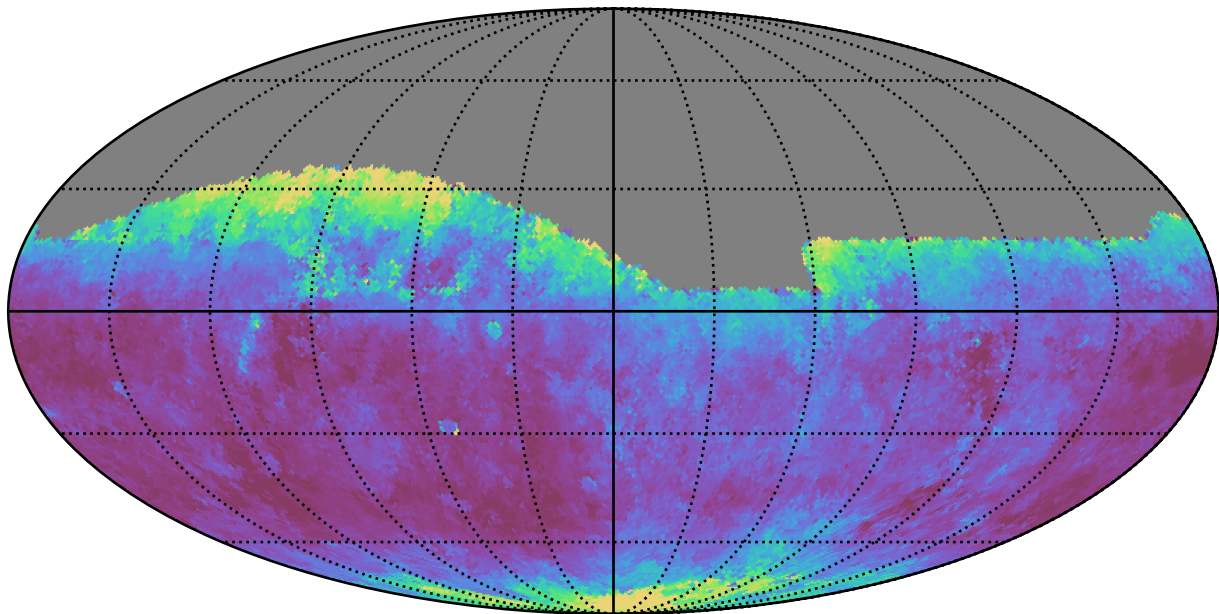
no_long_daily_v3.4_10yrs Yr 1 all bands: Median seeingEff
