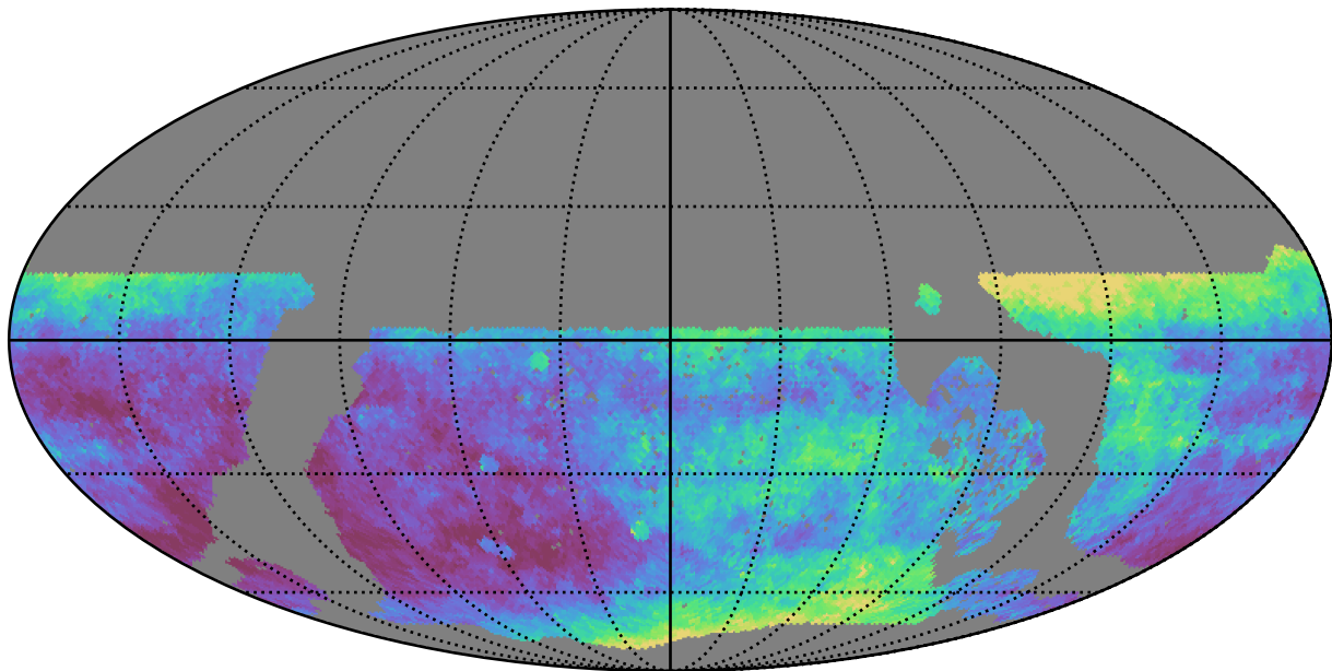
no_long_daily_v3.4_10yrs WFD z band: Median seeingEff
