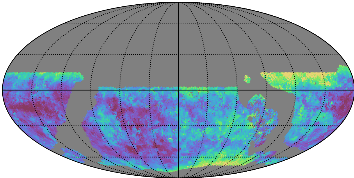
no_long_daily_v3.4_10yrs WFD u band: Median seeingEff
