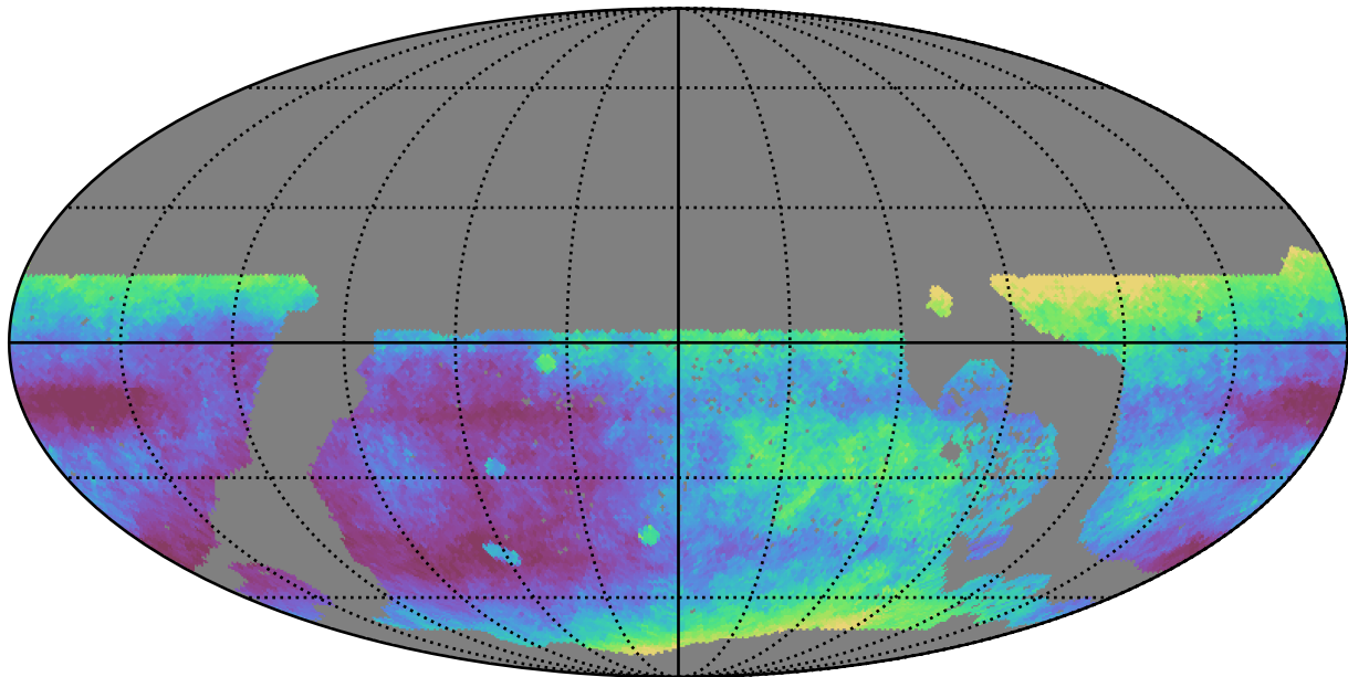
no_long_daily_v3.4_10yrs WFD r band: Median seeingEff
