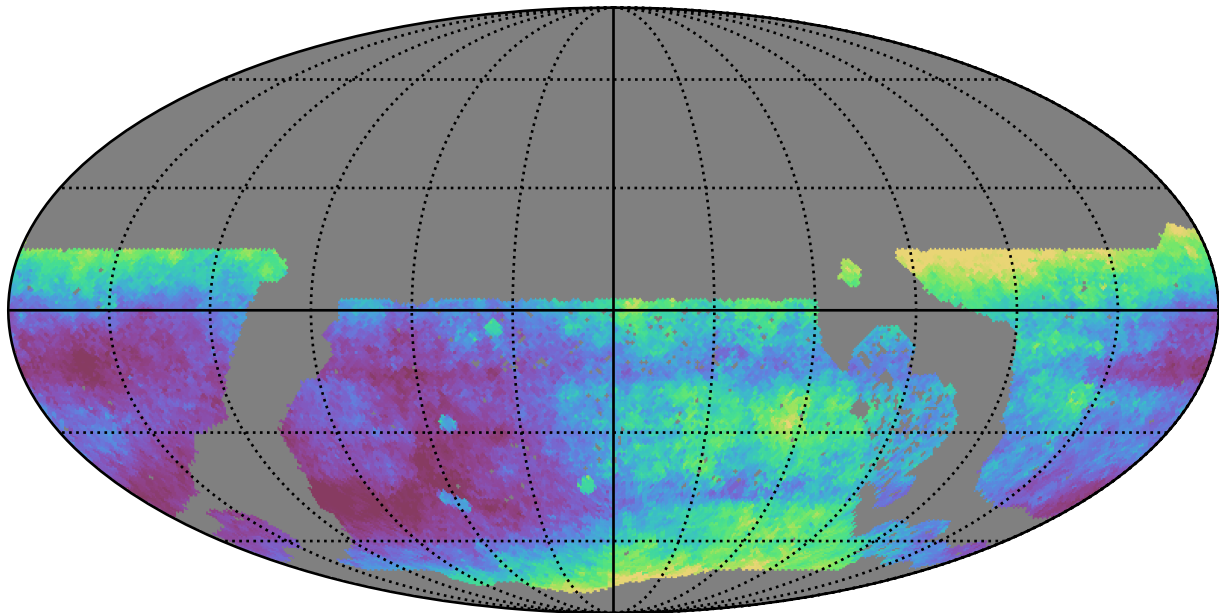
no_long_daily_v3.4_10yrs WFD i band: Median seeingEff
