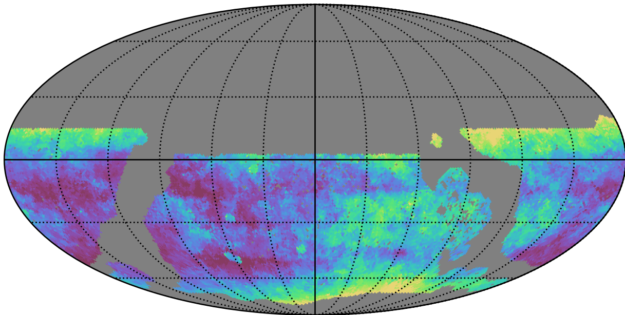
no_long_daily_v3.4_10yrs WFD g band: Median seeingEff
