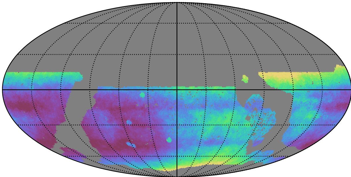
no_long_daily_v3.4_10yrs WFD all bands: Median seeingEff
