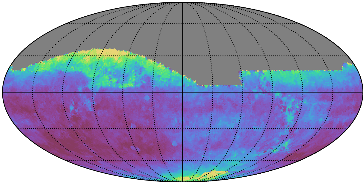
no_long_daily_v3.4_10yrs All sky z band: Median seeingEff
