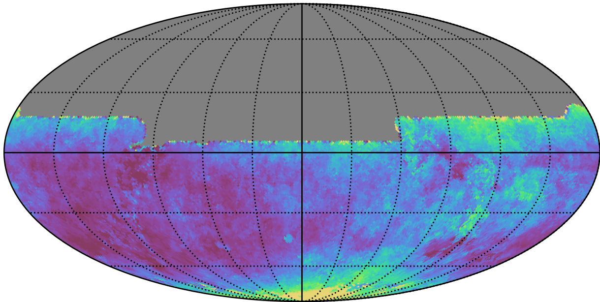
no_long_daily_v3.4_10yrs All sky y band: Median seeingEff
