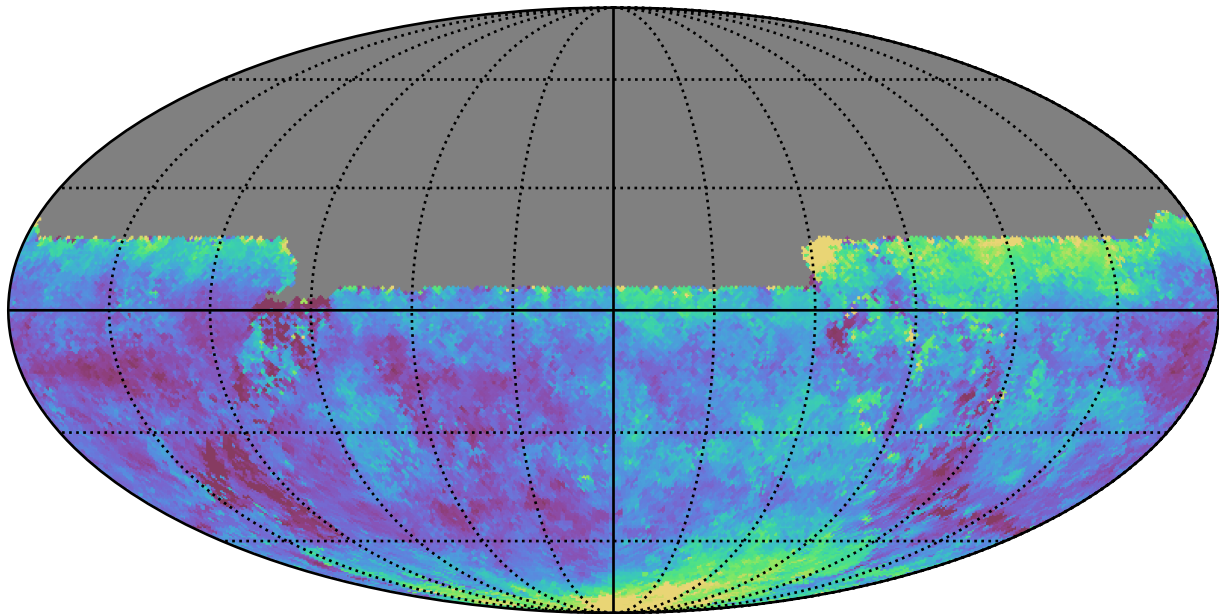
no_long_daily_v3.4_10yrs All sky u band: Median seeingEff
