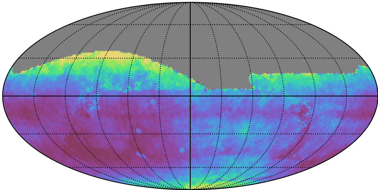
no_long_daily_v3.4_10yrs All sky i band: Median seeingEff
