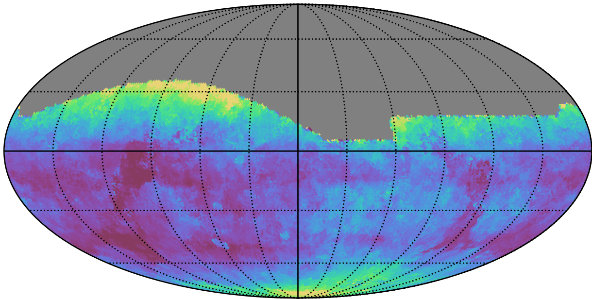
no_long_daily_v3.4_10yrs All sky g band: Median seeingEff
