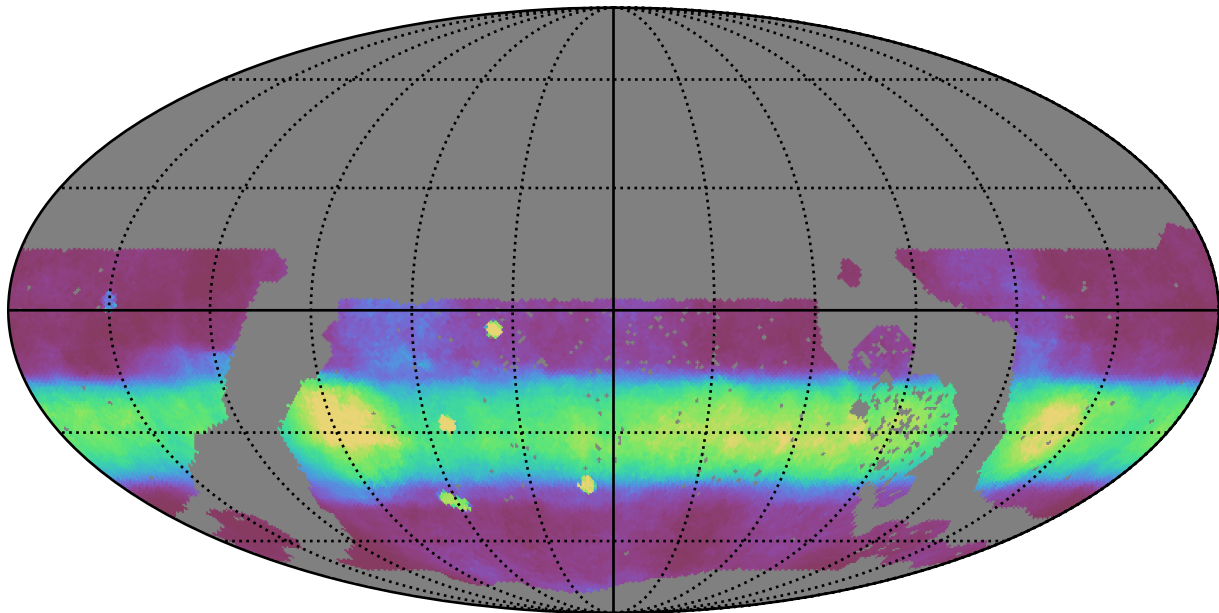
no_long_daily_v3.4_10yrs WFD all bands: Median normairmass
