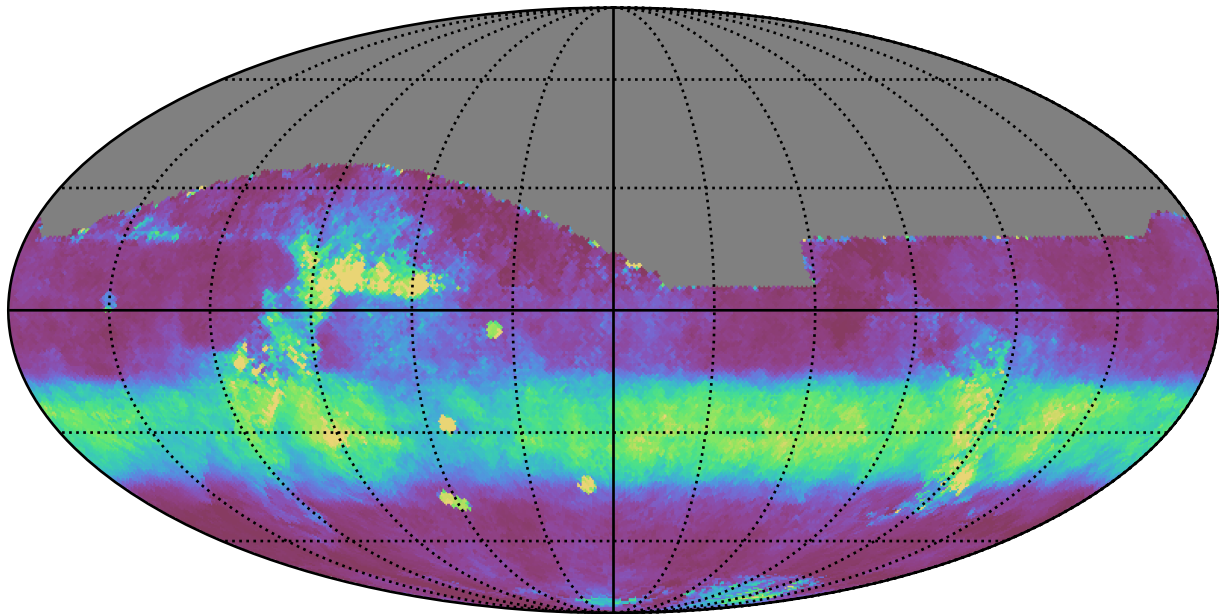
no_long_daily_v3.4_10yrs All sky z band: Median normairmass
