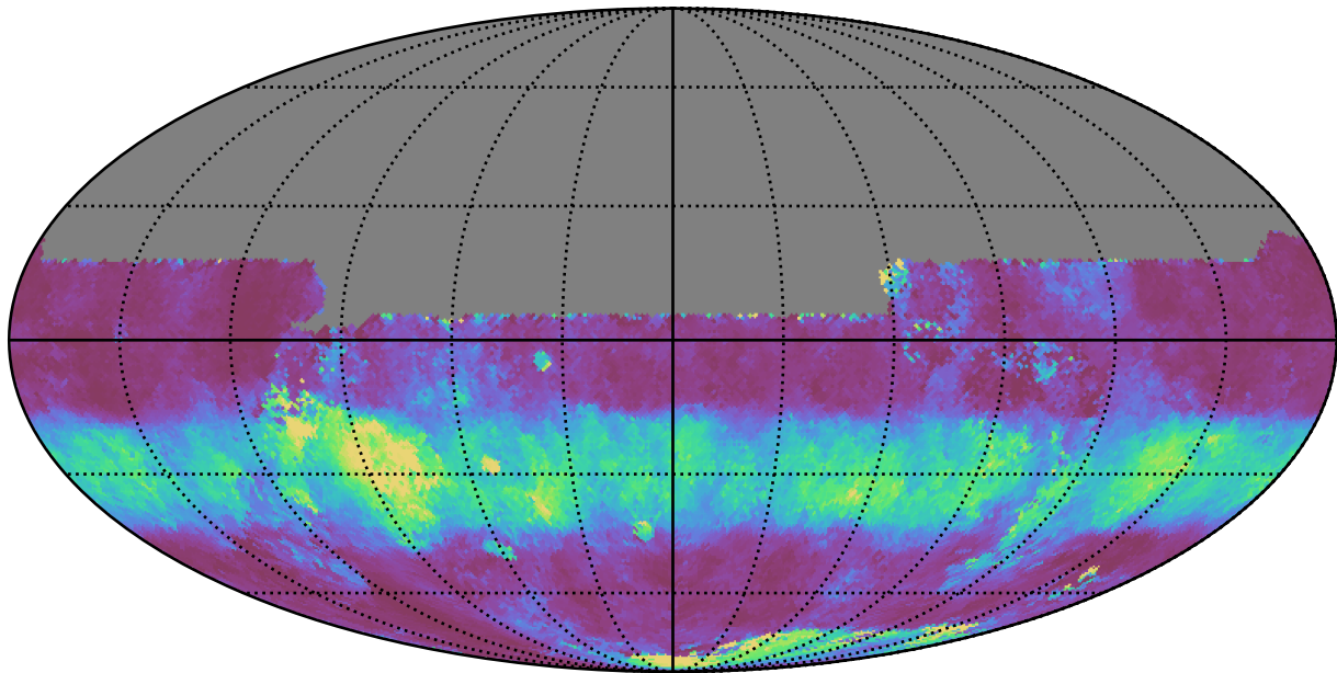
no_long_daily_v3.4_10yrs All sky u band: Median normairmass
