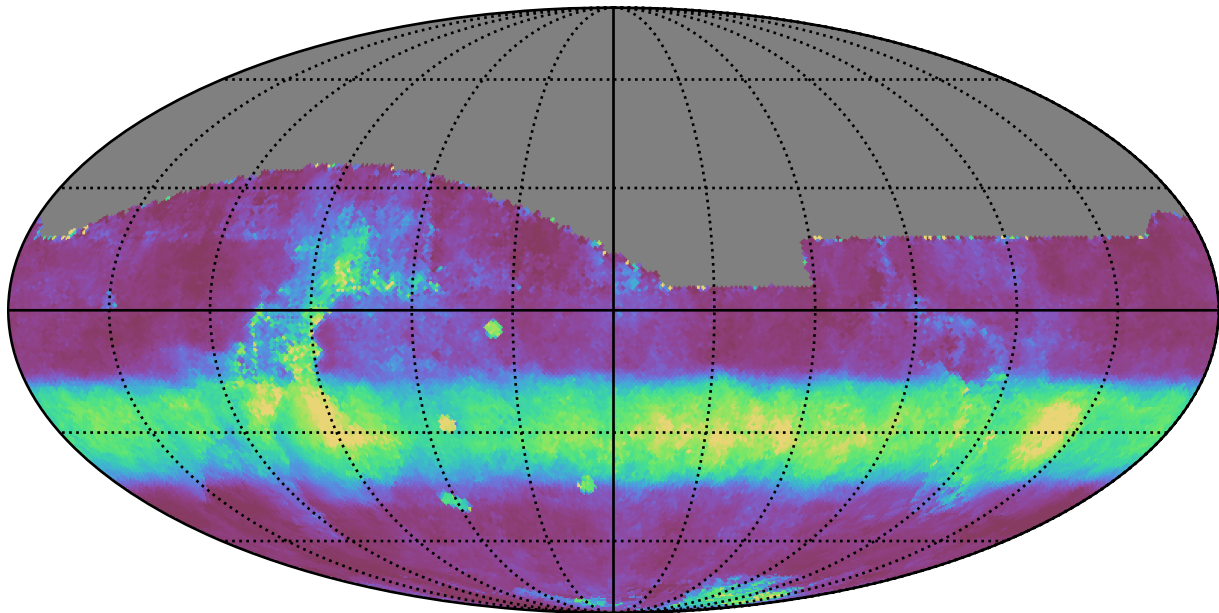
no_long_daily_v3.4_10yrs All sky i band: Median normairmass
