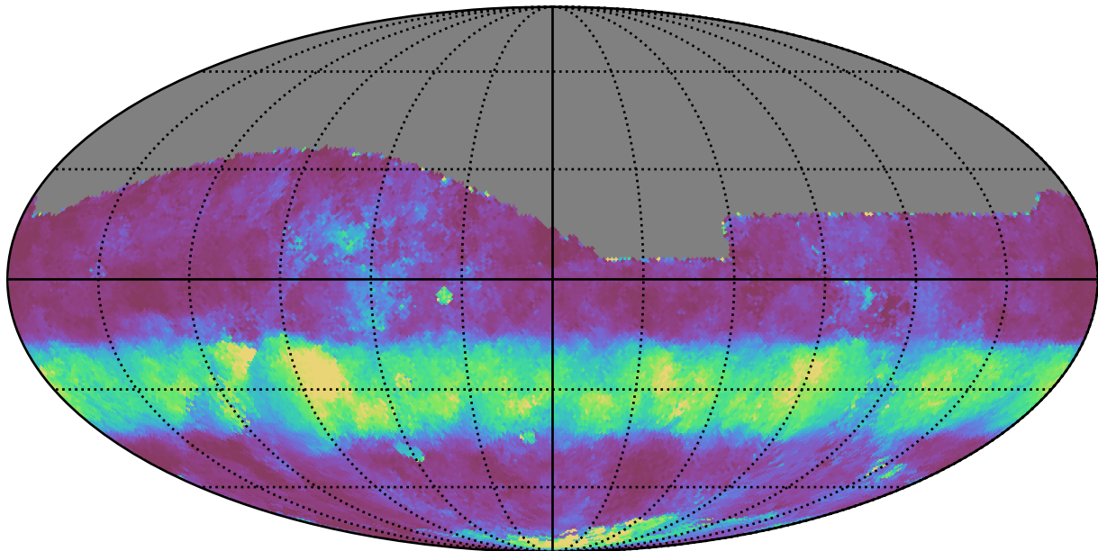
no_long_daily_v3.4_10yrs All sky g band: Median normairmass
