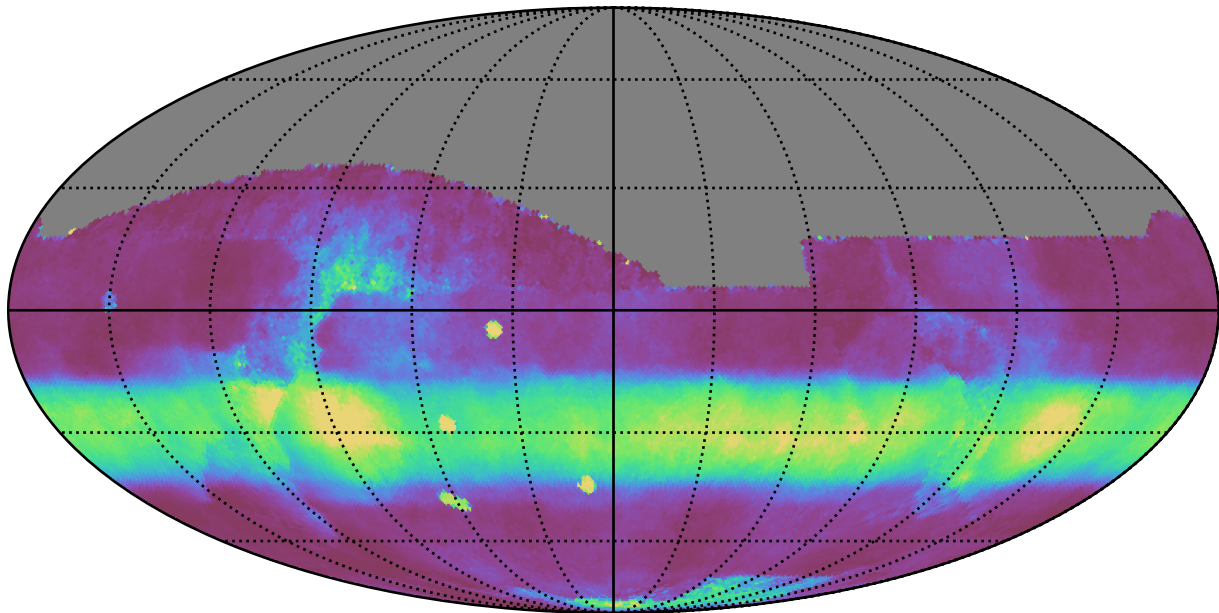
no_long_daily_v3.4_10yrs All sky all bands: Median normairmass
