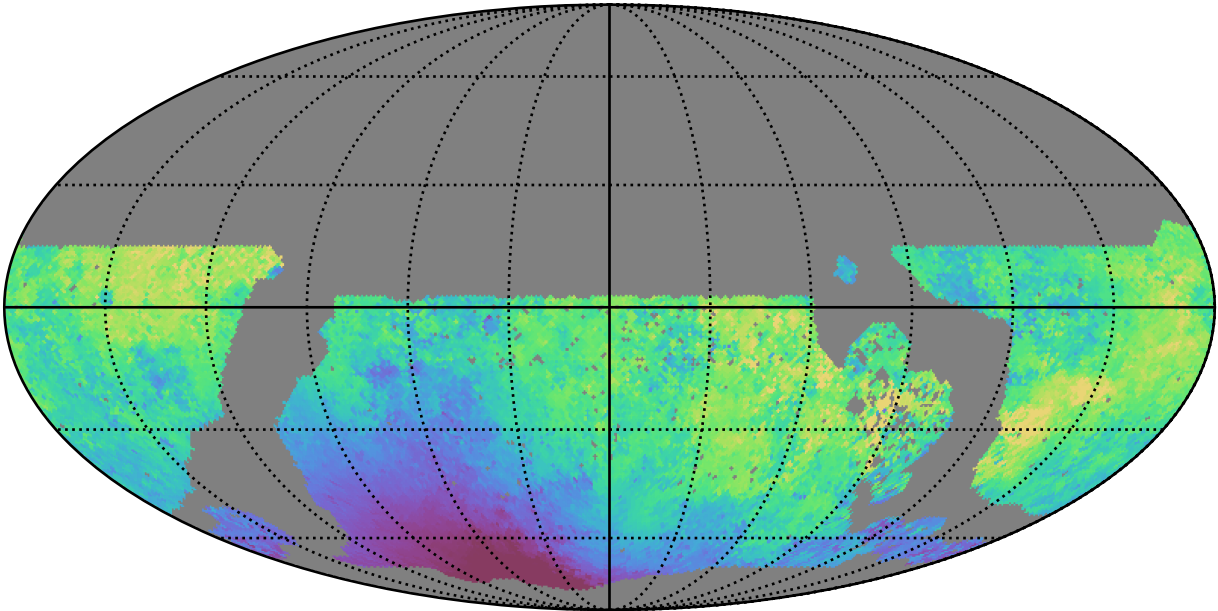
no_long_daily_v3.4_10yrs WFD u band: Median moonDistance
