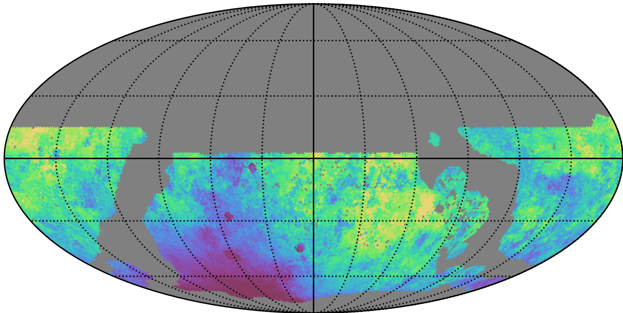
no_long_daily_v3.4_10yrs WFD r band: Median moonDistance
